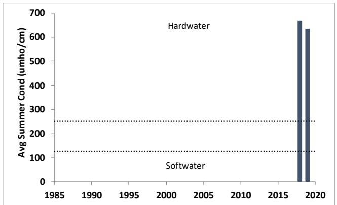
Specific Conductance
